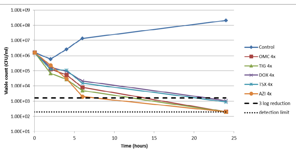
Figure 3. Time-kill of omadacycline and comparators against H. influenzae 977279.
