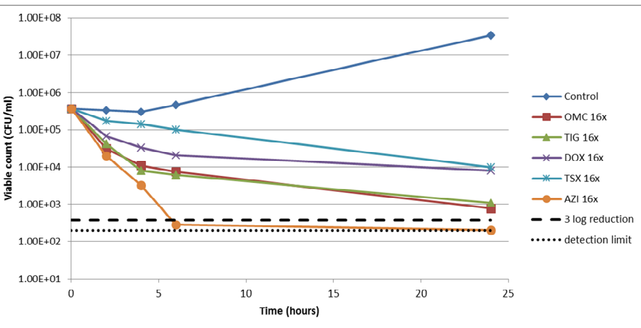
Figure 5. Time-kill of omadacycline and comparators against M. catarrhalis 943604.
