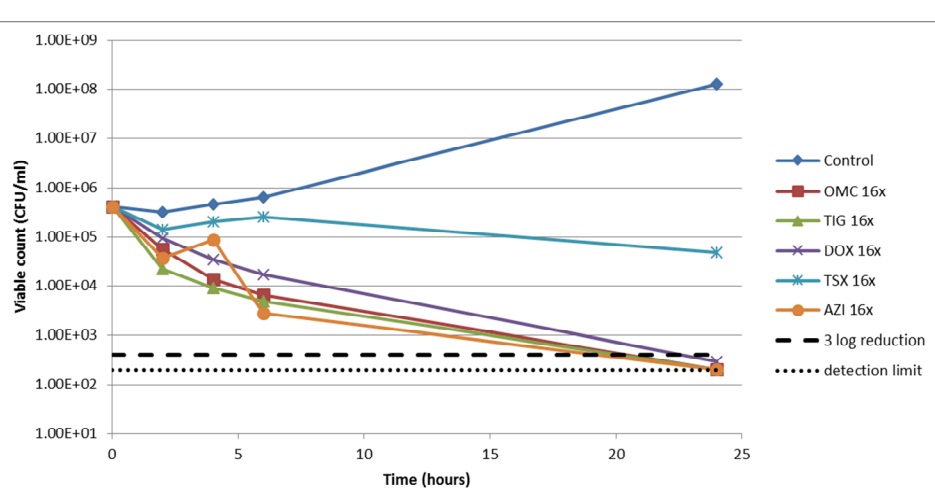
Figure 6. Time-kill of omadacycline and comparators against M. catarrhalis 953887.
